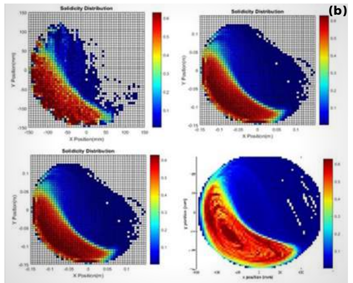
Fig. 2: (a) Comparison of tangential velocity of charge particle (obtained from EDEM) predicted by different models against PEPT data and (b) Predicted solidicity comparison. Top: (Left: DEM, Right: One-way coupling), Bottom: (Left: Two-way coupling, Right: PEPT experimental results) for the total mill volume filling of 31.25% with charge and slurry containing 20% solids.
