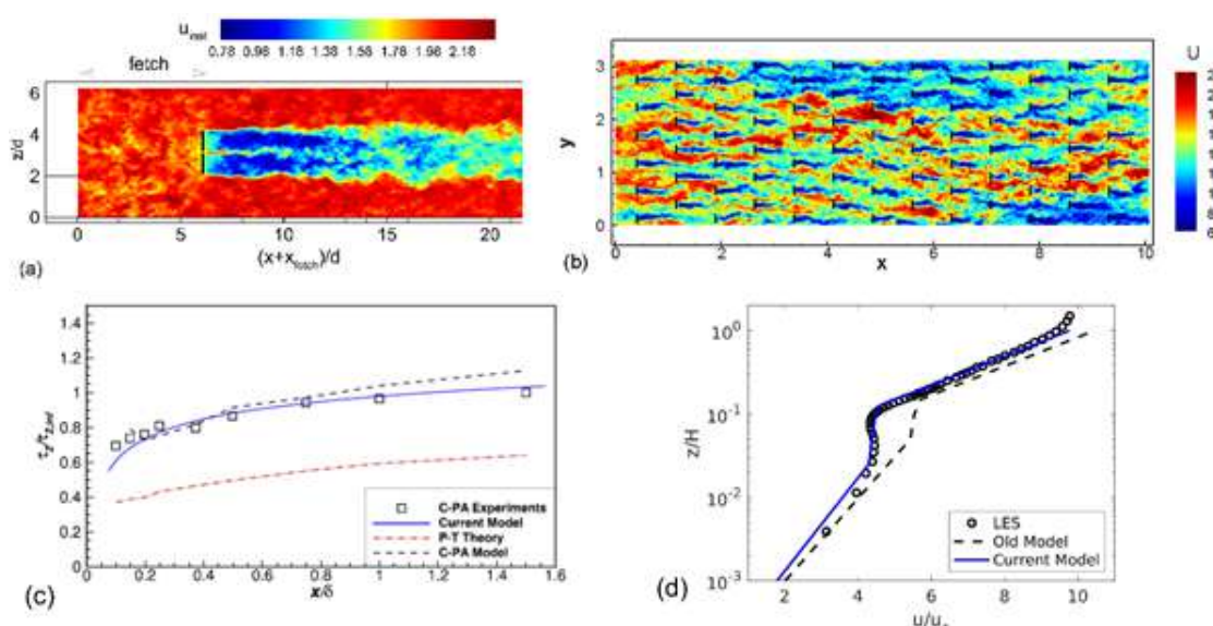
Fig. 8: Contours of the instantaneous velocity field behind (a) a stand-alone multi-rotor wind turbine, (b) a very large wind farm. Thick black lines denote turbine rotors. Analytical model predictions for (c) the shear stress behind a surface roughness jump compared to previous models and experiments and (d) mean velocity profile in very large wind-farms compared to a previously proposed model and LES results
